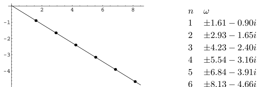
Figure 12: The spectrum of the first twelve quasi-normal vector modes of the chirally symmetric phase of the Sakai-Sugimoto model (each mode is twofold degenerate because of chiral symmetry).
